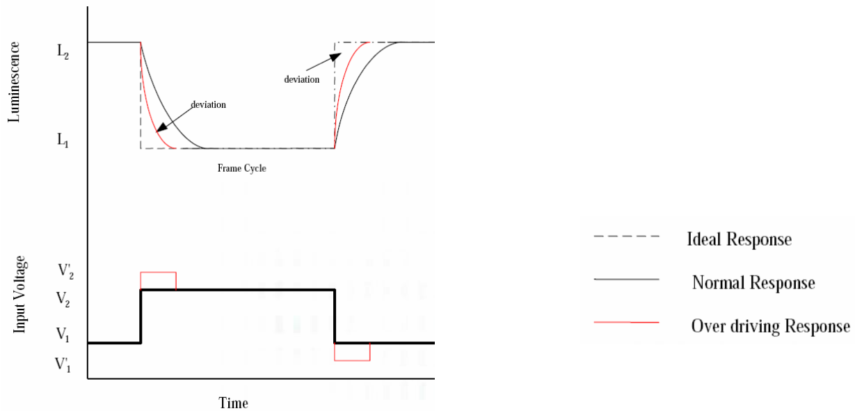
Figure 3: Amplified Impulse Overdrive Scheme
